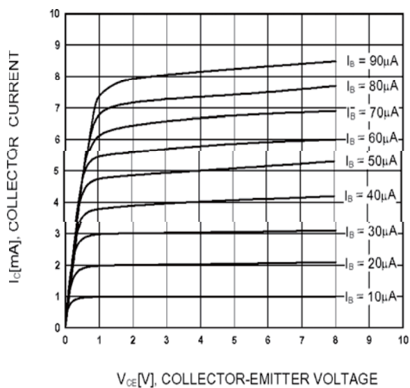
Static Characteristic
